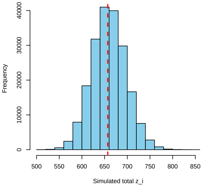
Simulated vs Observed Total Deaths
