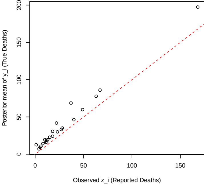
Observed vs. Posterior Expected True Deaths
