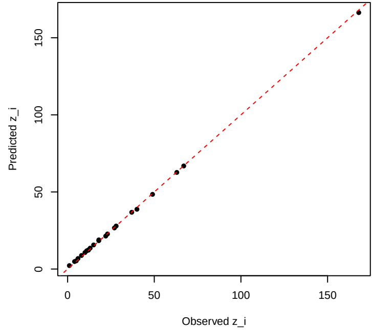
Observed vs Expected Reported Deaths by LGA
