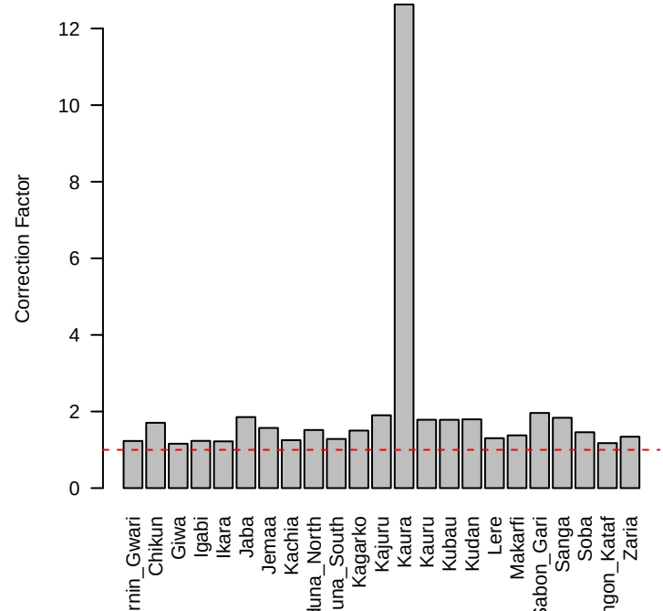
Implied Under-reporting Adjustment: y_i / z_i
